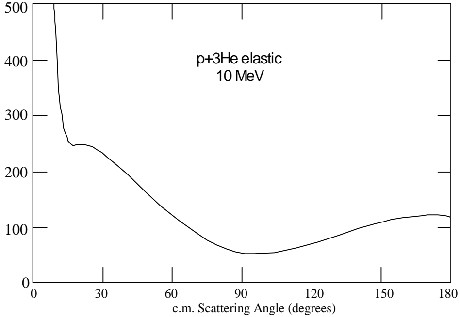
Figure 6.1 Example of Chargewd-Particle Elastic Scattering Cross Section
